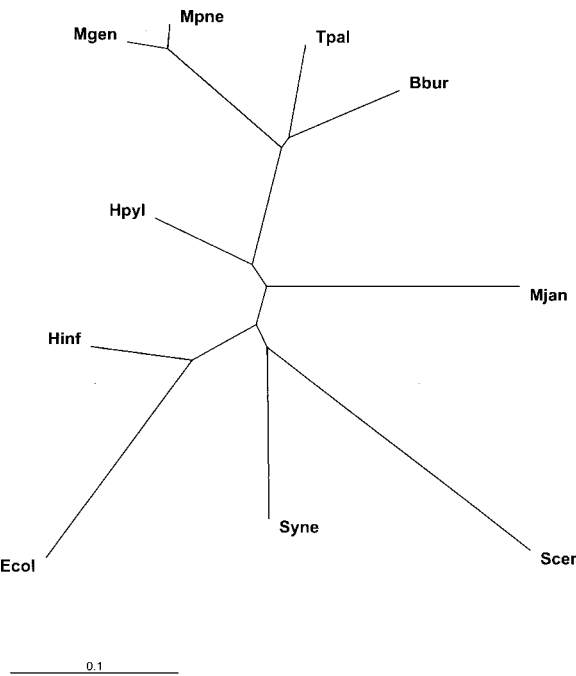
Figure 3. A phylogenetic tree of 10 completely sequenced organisms, including T. pallidum and B. burgdorferi . The tree was constructed based on the pairwise similarity between the fold contents of the genomes.
