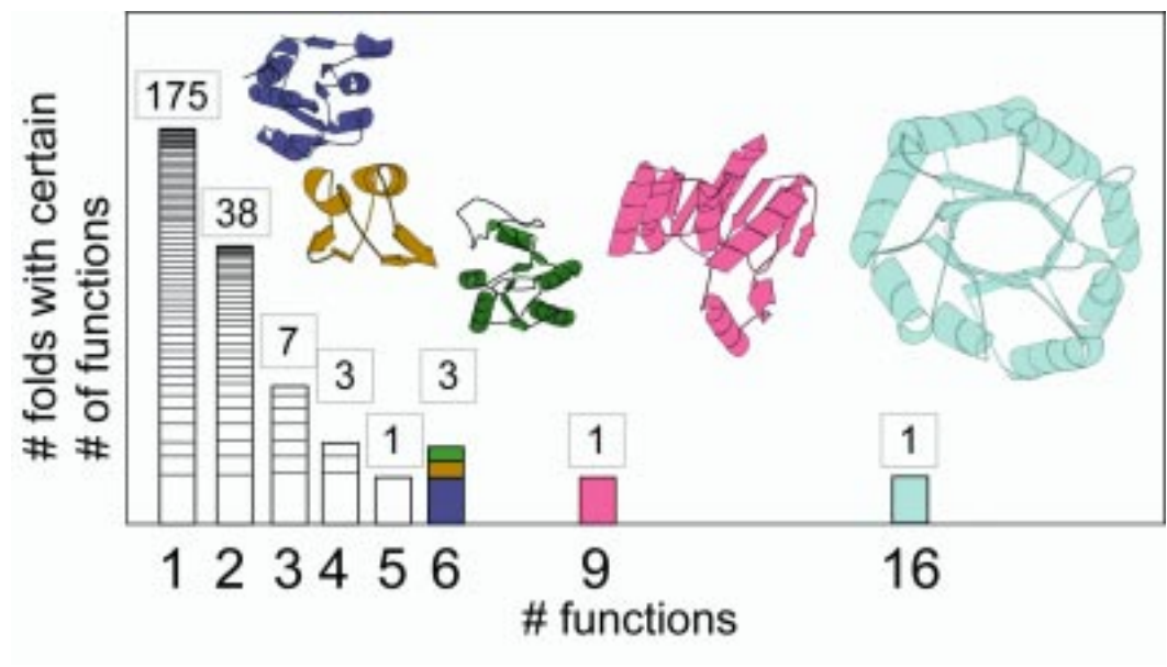
Figure 1. The functional distribution of the most diverse folds occurring in Swissprot. The X-axis indicates the number of functions, and the Y-axis denotes the number of folds that have been associated with that many functions. A schematic is shown for each of the 5 functionally most diverse folds.
