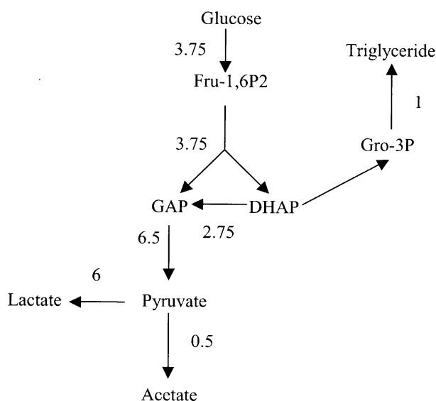
Figure 6. Flux values for the reactions as obtained by Flux-Balancing Method. Those reactions, for which flux values are zero, are not shown in the figure. In the flux analyses we have optimized the values of reaction rates subject to the condition of minimum glucose uptake. Examples of equations, for the reaction intermediates, solved by the optimization procedure:
