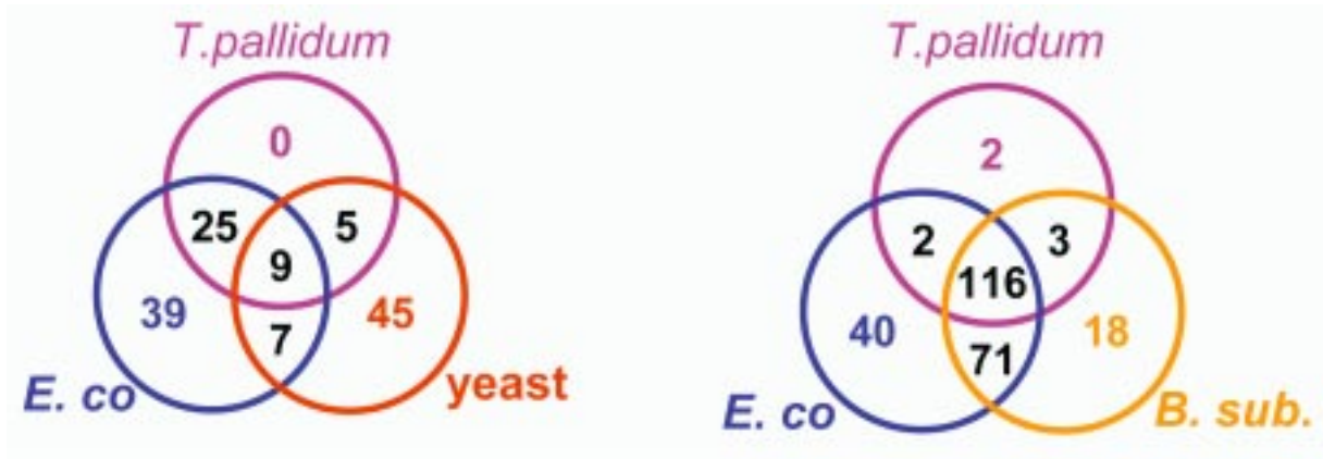
Figure 2. Two Venn-diagrams, showing the number of shared and unique folds among T. pallidum , E.coli and yeast (on the left-hand side), and among T. pallidum , E. coli and Bacillus subtilis .
