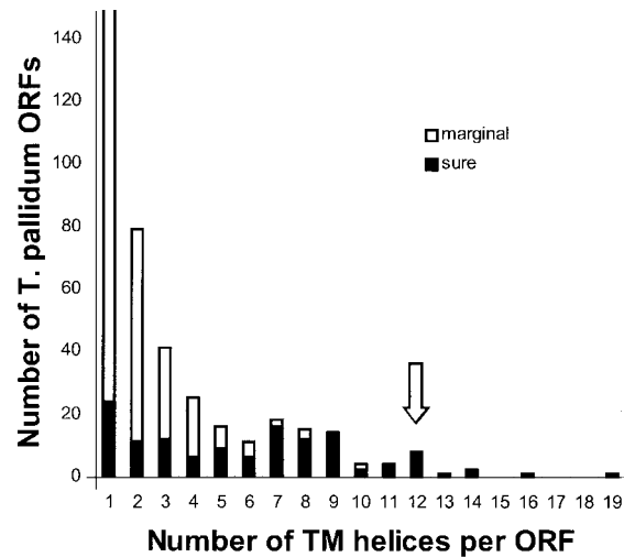
Figure 4. Distribution of the ORFs with transmembrane helices in T. pallidum with respect to the number of helices per ORF. The highest number of TM-helices was found to be 19, detected only in one ORF.
