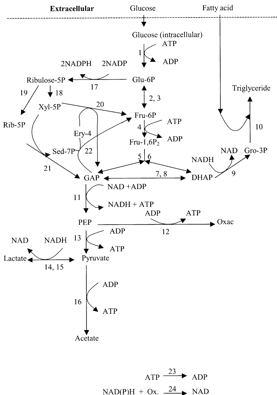
Figure 5. Simplified metabolic model for glucose and lipid metabolism in T. pallidum and B. burgdorferi . Reaction-numbers are numbered shown beside the arrows. Abbreviations used for the metabolites are as follows: Glu-6P (Glucose-6-phosphate), Fru-6P (Fructose-6-phosphate), Fru-1,6P2 (Fructose-1,6-biphosphate), GAP (Glyceraldehydes phosphate), DHAP (Di-hydroxy acetone phosphate), PEP (Phosphoenol pyruvate), Gro-3P (Glycerol-3-phosphate), Oxac (Oxaloacetate). Glucose and fatty acids are transported into cell from the extracellular medium. Since water forming NADH oxidase is present in both the organism, NADH is oxidized to NAD + in the spirochetes as shown in reaction 24.
