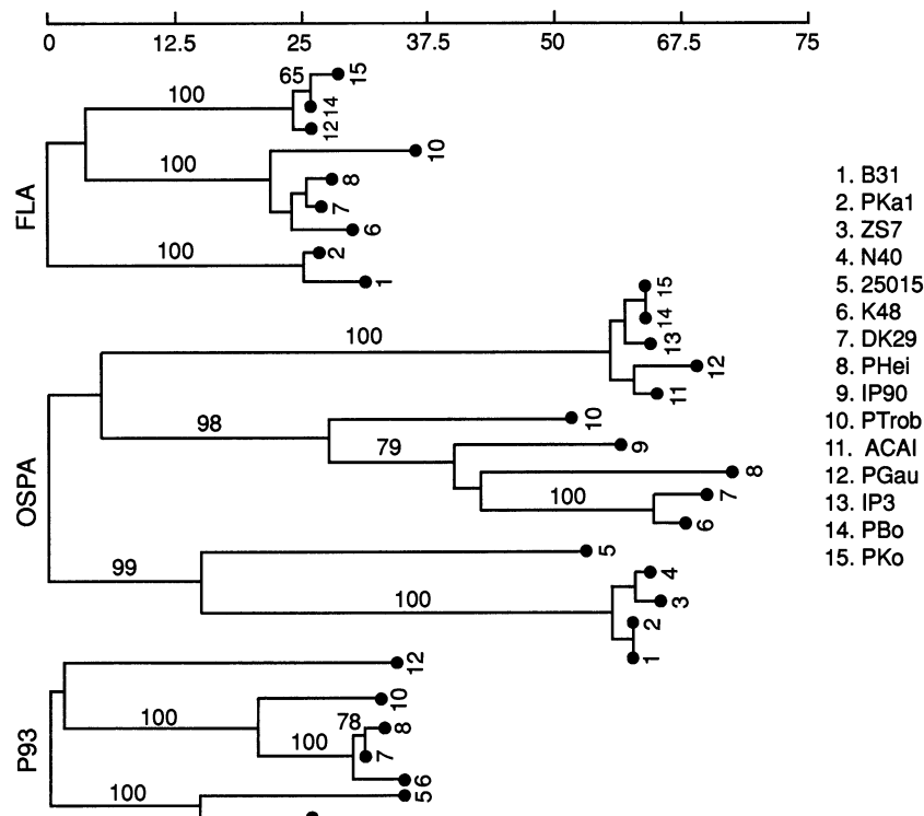
FIG. 1. Phylogenetic trees from the DNA sequences of p93 , ospA , and fla . The scale is in changes per kilobase of DNA. The trees were generated by using the neighbor-joining (32) option on NTSYS-pc (33). The input distance matrix for each tree was the number of mismatches in the DNA sequence for each pair. The trees were rooted by midpoint rooting. The branch lengths were normalized to changes per kilobase of DNA for the figure. Thus, the trees are comparable as to rate. Strains represented as the ends of a straight line have the identical sequence. The numbers on the branches are the percent of trees retaining the cluster when the data is bootstrapped. The neighbor-joining trees were compared to trees generated by maximum parsimony using the program PAUP (30) and were found to be congruent. The neighbor-joining trees were better defined—i.e., undefined tricotomies by maximum parsimony were defined by neighbor joining. The bootstrap analysis was done by using maximum parsimony, giving a conservative estimation of the stability of nodes.
